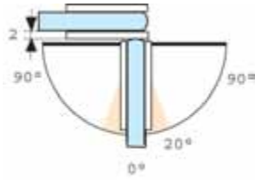
Glas/Glas 4 mm Luft Glass/Glass 4 mm gap
